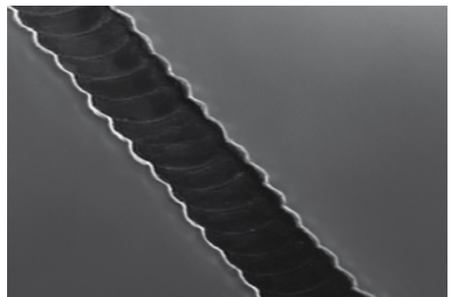
Figure 2: Scribing of Molybdenum (CIS P1), track width approx. 45 μm
