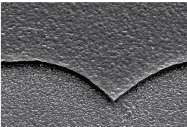
Figure 1: Removal of aSi/μSi-absorber and metal back contact without damaging TCO-layers underneath (aSi/μSi P3)
